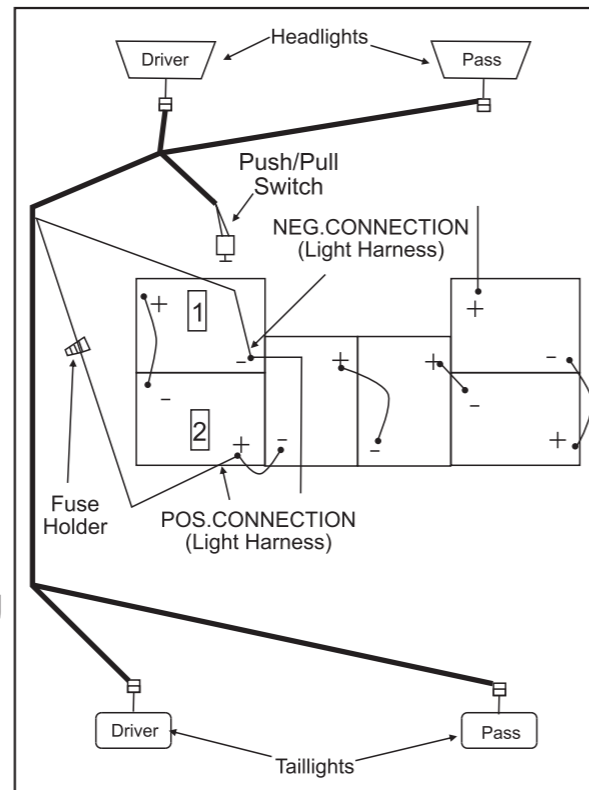
Club Car Basic 36-Volt Wiring Diagram
